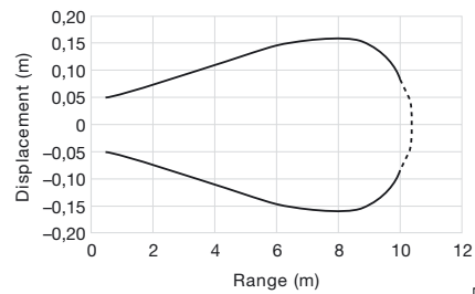
SPPR 2x10
