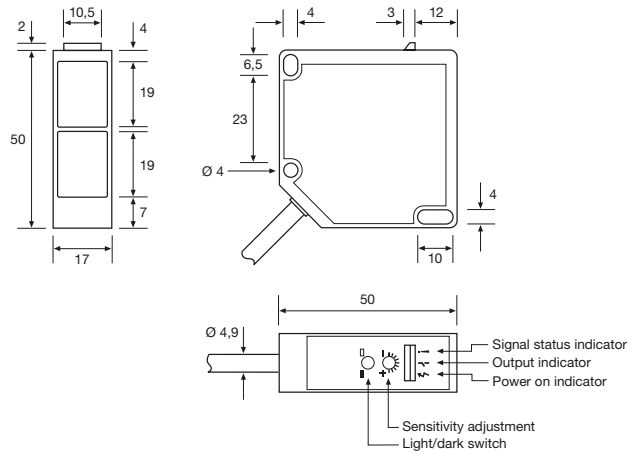
SPR/SPP/SPRR/SPPR/SPBS 2xxx 5
