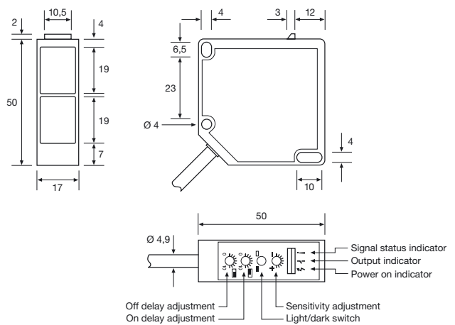
SPR/SPP/SPRR/SPPR/SPBS 2xxxT 5
