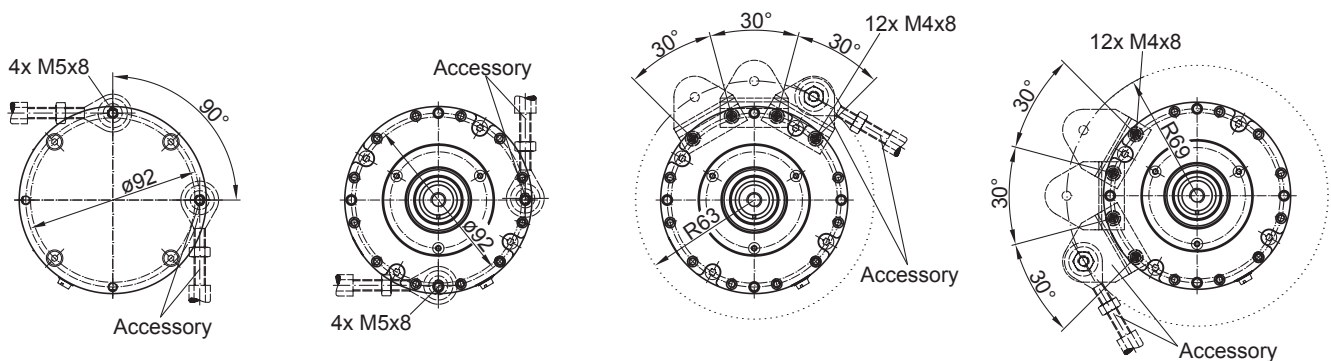
Mounting possibilities
